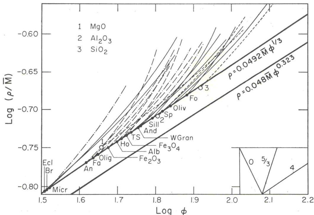
Fig. 2. As in Figure 1 for adiabats derived using equation 6. Solid straight line is revised seismic equation of state line, equation 6. Solid straight line of equation 5 is also shown.
